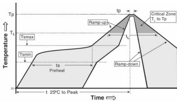
Figure 5. Reflow Profile
